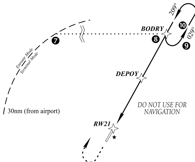
Figure 6-29 Terminal Mode
