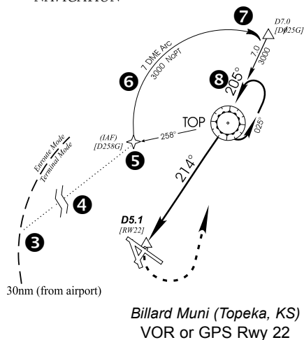
Figure 6-40 Terminal Mode
