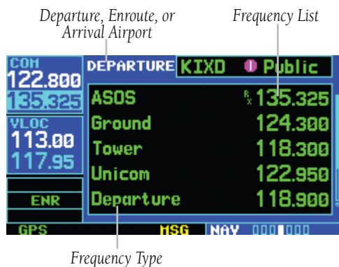
Figure 1-20 NAV/COM Page
