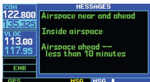
Figure 1-29 Messages Page
