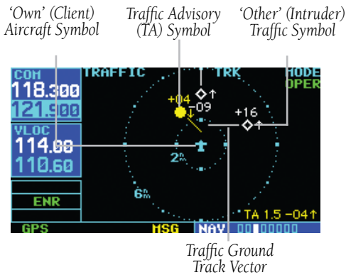
Figure 12-2 Traffic Page
