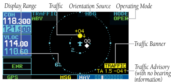
Figure 12-23 Traffic Page
