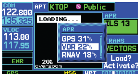
Figure 6-39 Approach Window
