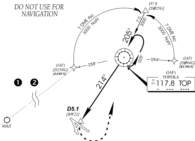
Figure 6-36 Enroute Mode
