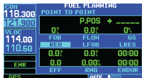
Figure 10-12 REQ Highlighted
