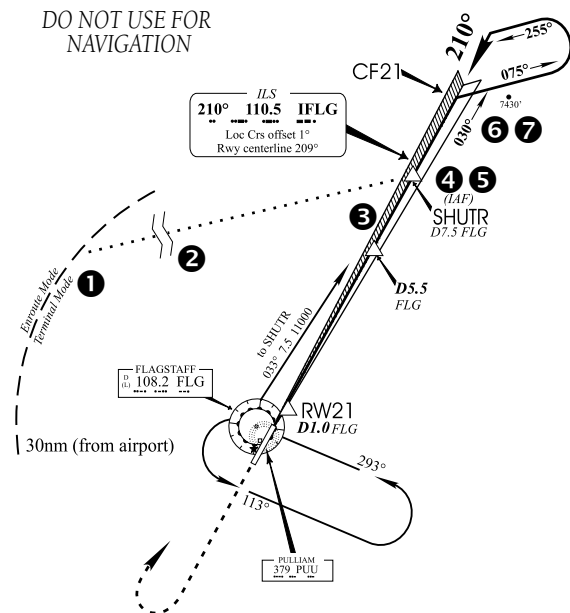
Figure 6-77 Terminal Mode
