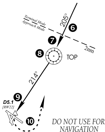
Figure 6-55 Approach Mode
