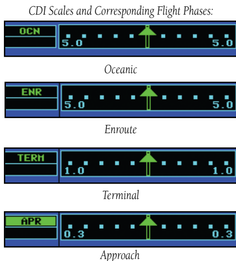
Figure 10-54 CDI Scales
