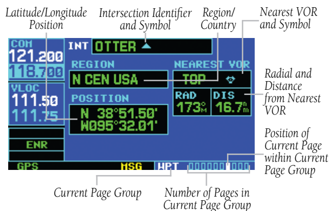
Figure 7-31 Intersection Page
