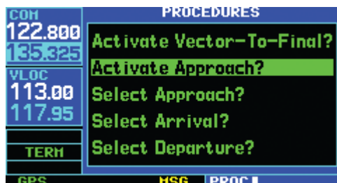
Figure 6-78 Activate Approach
