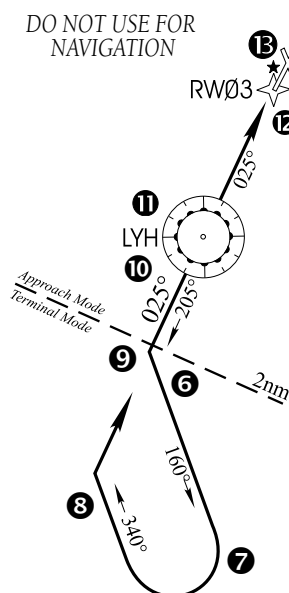
Figure 6-16 Terminal Mode
