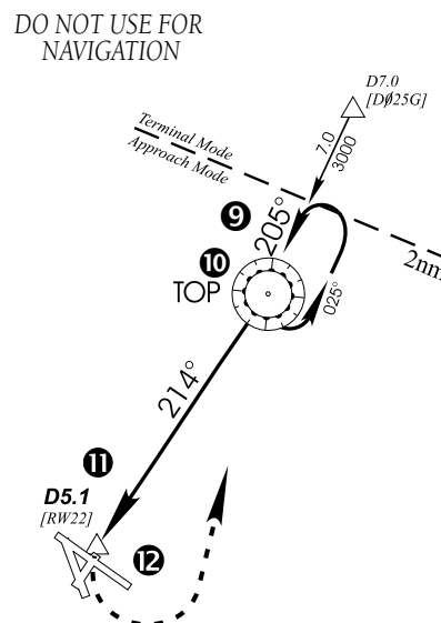
Figure 6-44 Approach Mode
