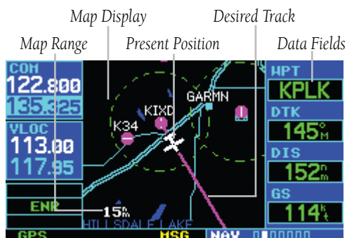
Figure 1-14 Map Page
