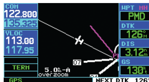
Figure 6-67 Waypoint Alert
