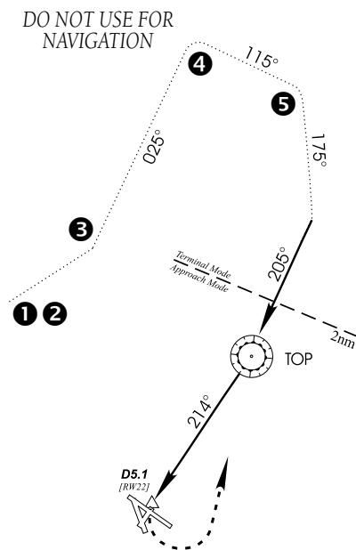
Figure 6-51 Terminal Mode
