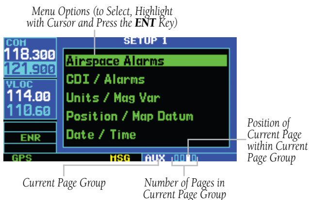
Figure 10-51 Setup 1 Page
